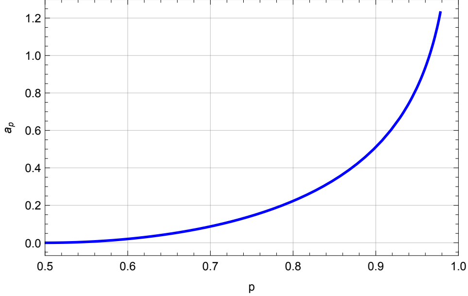
FIGURE 2. When given signals with strength p , an agent who does not observe the other agent chooses the wrong action at time n with probability e^{-a_p \cdot n + o(n)} , where a_p = D_{KL}(1/2 || p) .
